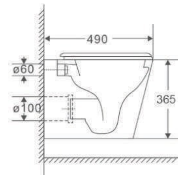
Calma Wall Hung Water Closet
