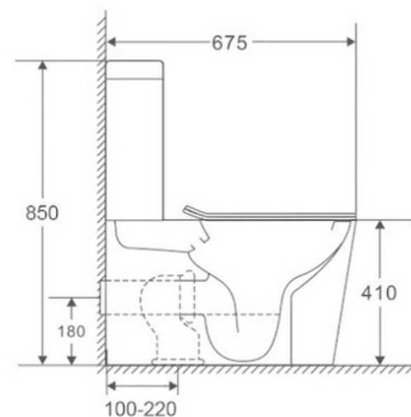
Calma Water Closet
