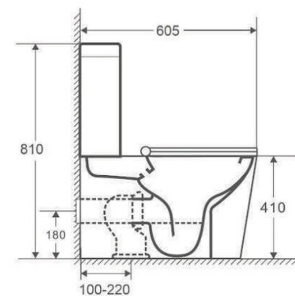
Calma S Water Closet
