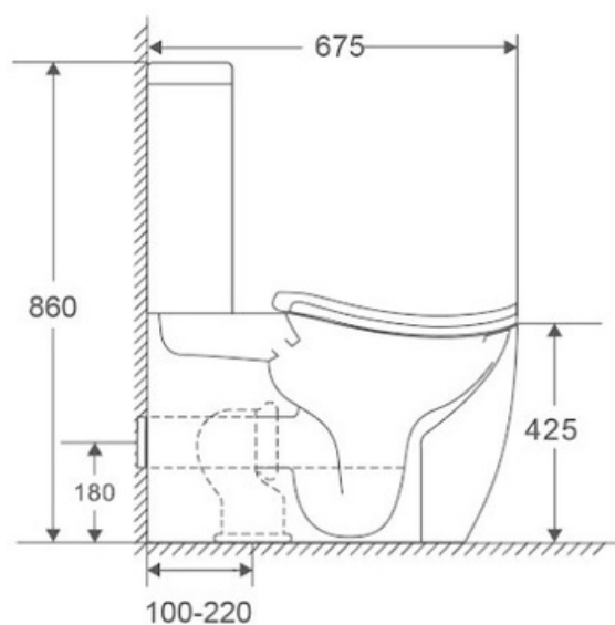
Argo Water Closet
