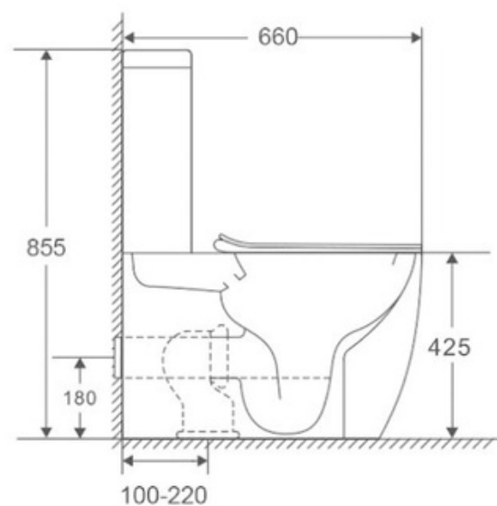
Lumina Water Closet
