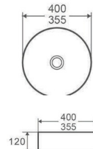
Prism S Wash Basin RB.TGN.OBW130.CE.PB
