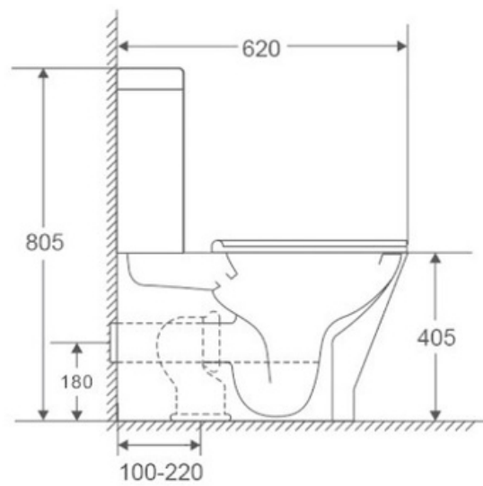
Viva Water Closet
