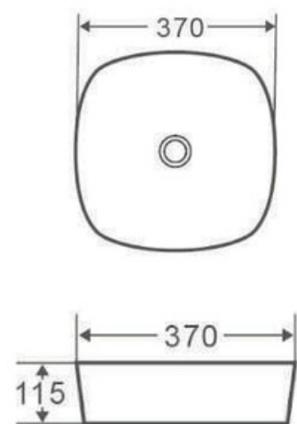
Aura 370 Wash Basin RB.TGN.OBW130.CE.PD
