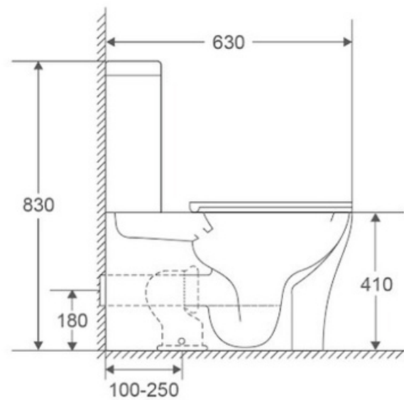
Nivele Water Closet
