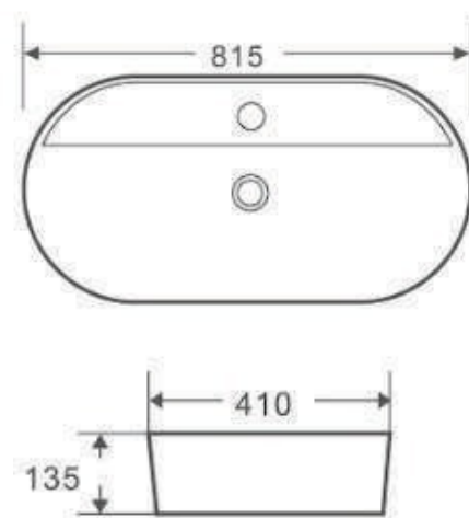
Florina 204 Wash Basin RB.TGN.OBW130.CE.PK
