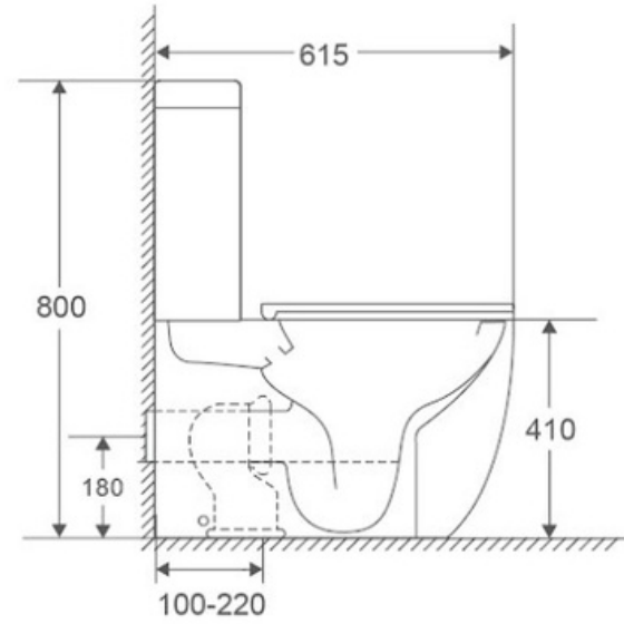
Velo Water Closet
