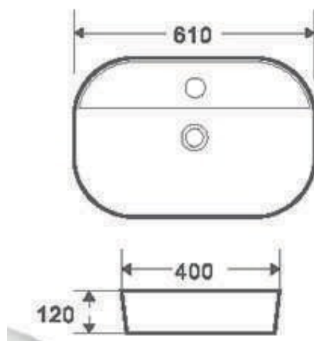
Florina 203 Wash Basin RB.TGN.OBW130.CE.PN
