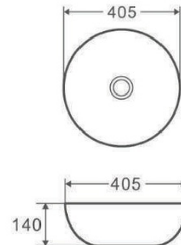
Iris Wash Basin RB.TGN.OBW130.CE.PM
