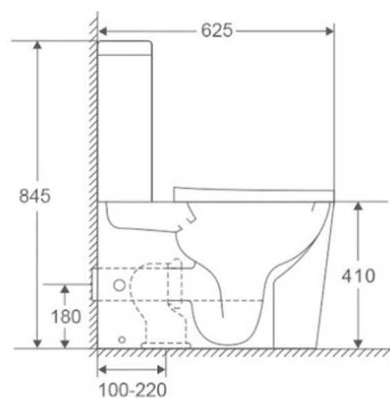
Solana Water Closet
