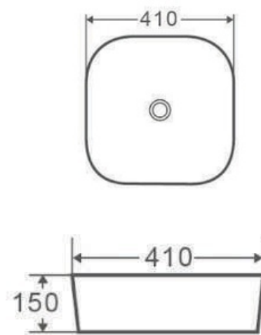
Aura 410 Wash Basin RB.TGN.OBW130.CE.PF
